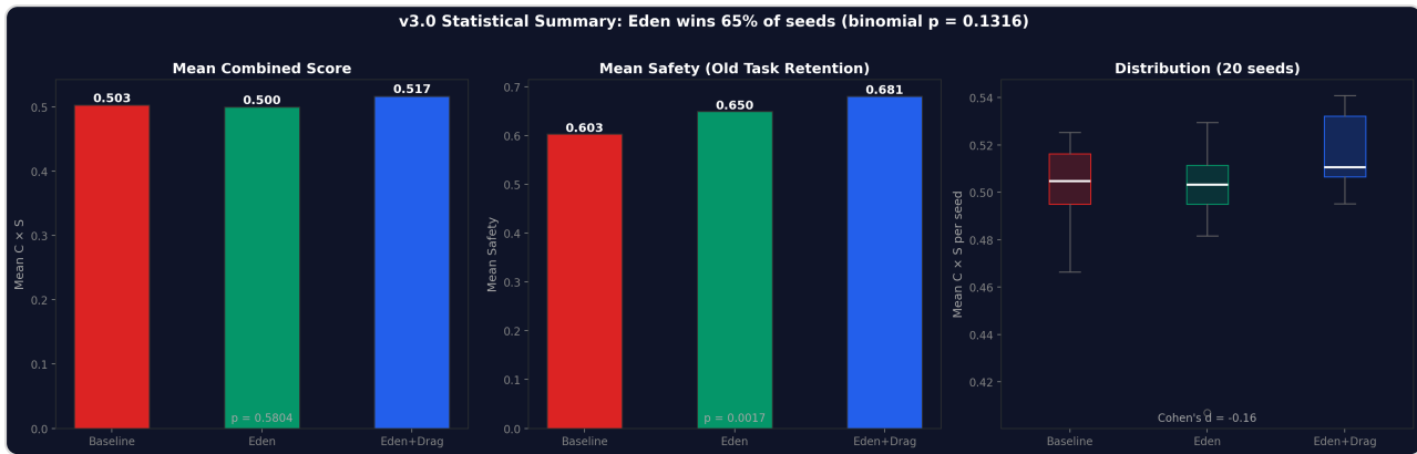
Figure 6. v3 adversarial statistical summary across 20 seeds.
