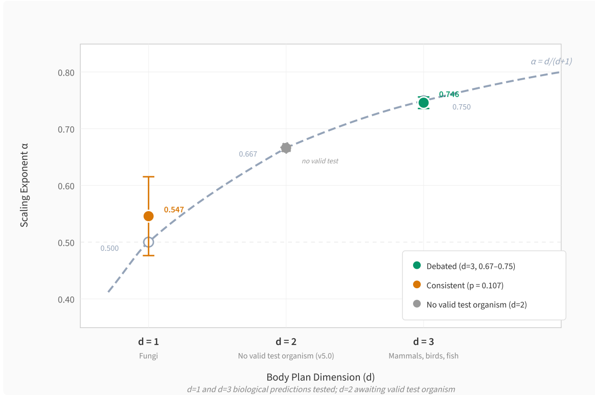
Figure 2 | The Dimensional Ladder. Dashed curve: \alpha = d/(d+1) , independently derived by West et al. [ 17 , 21 ],
