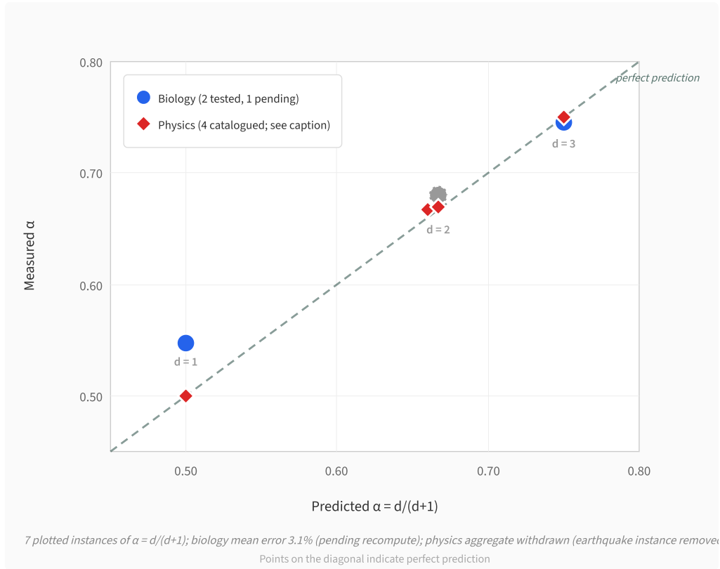
Figure 3 | Predicted vs Measured. Cross-domain instances of one independently derived formula: \alpha = d/(d+1) [ 17 , 21 , 22 , 23 ,24, 25 ]. Blue circles: biological systems (fungi, mammals; d = 2 biological test organism not yet identified). Red diamonds: physics systems (crystal growth, phase transitions, fracture; earthquake data point removed; retained separately as a variable-pair case study in the text). Points on or near the diagonal indicate accurate prediction. A single equation, with zero adjustable parameters, governs systems spanning biology, geophysics, and condensed matter physics. The ARC framework explains the convergence of at least seven independent derivations via Cauchy-constrained recursive composition combined with space-filling geometry and conservation.
