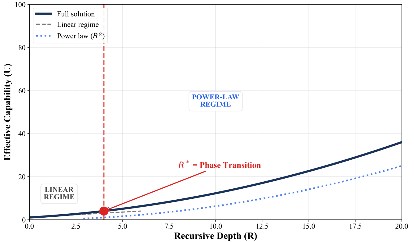
Figure 14 | The Scaling Crossover at R^* . Below the critical depth R^* , base capability ( I ) dominates and scaling appears linear. Above R^* , recursive compounding dominates and scaling becomes power-law. This crossover point is the depth at which recursive amplification becomes dominant. Systems should exhibit a distinct "elbow" in their capability curves at R^* .
