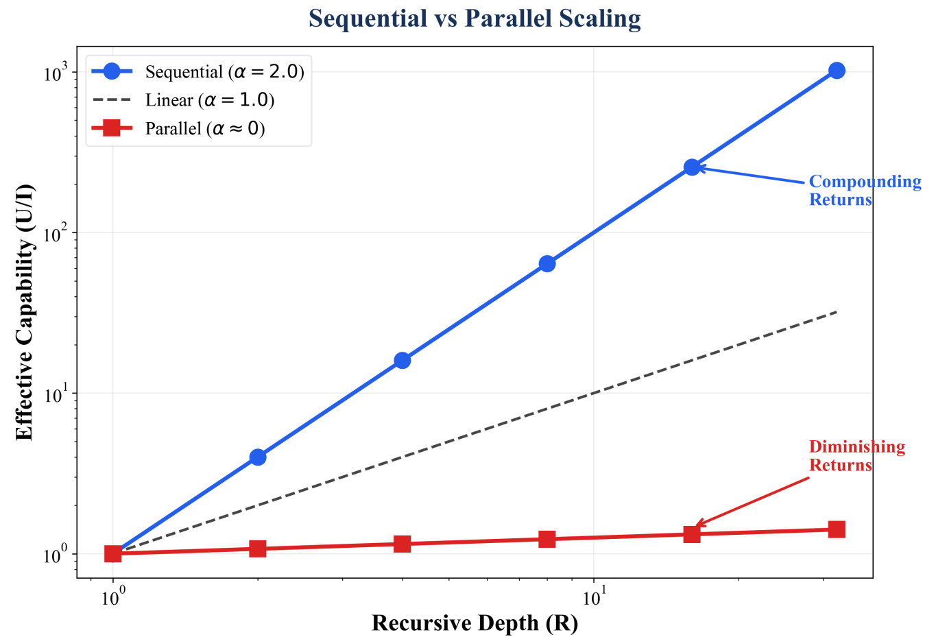
Figure 3 | Scaling Comparison. Log-log plot showing different scaling regimes. Power law U = R^\alpha appears as a straight line with slope \alpha . Sequential recursion ( \alpha > 1 ) shows super-linear growth; parallel sampling ( \alpha < 1 ) shows diminishing returns. The ARC Principle predicts \alpha_{\text{sequential}} > 1 > \alpha_{\text{parallel}} .
