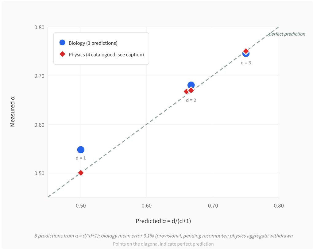
Figure 10 | Predicted vs Measured. Eight cross-domain predictions from one formula: \alpha = d/(d + 1) . Blue circles: biological systems (fungi at d=1 , jellyfish at d=2 , mammals at d=3 ). Note: the d=2 datum (jellyfish, measured \alpha = 0.680 ) is under review in the paper's later analysis (§3.6, §3.7); it is retained here as plotted evidence pending reconciliation of the 2D biology entry across sections. Red diamonds: physics systems (crystal growth, phase transitions, fracture; earthquake data point removed; retained separately as a variable-pair case study). Every remaining point falls on or near the diagonal of perfect prediction. A single equation, with zero adjustable parameters, governs systems spanning biology, geophysics, and condensed matter physics.
