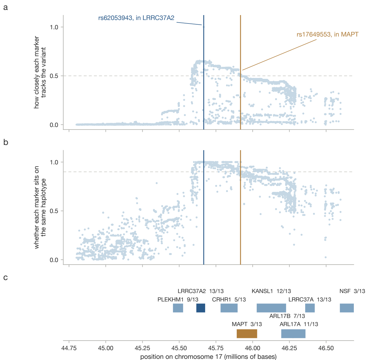
Supplementary Fig. 12 | Linkage disequilibrium of rs62053943 across chr17:44.8–46.6 Mb, as r^2 ( a ) and |D'| ( b ), with the gene track ( c ).
