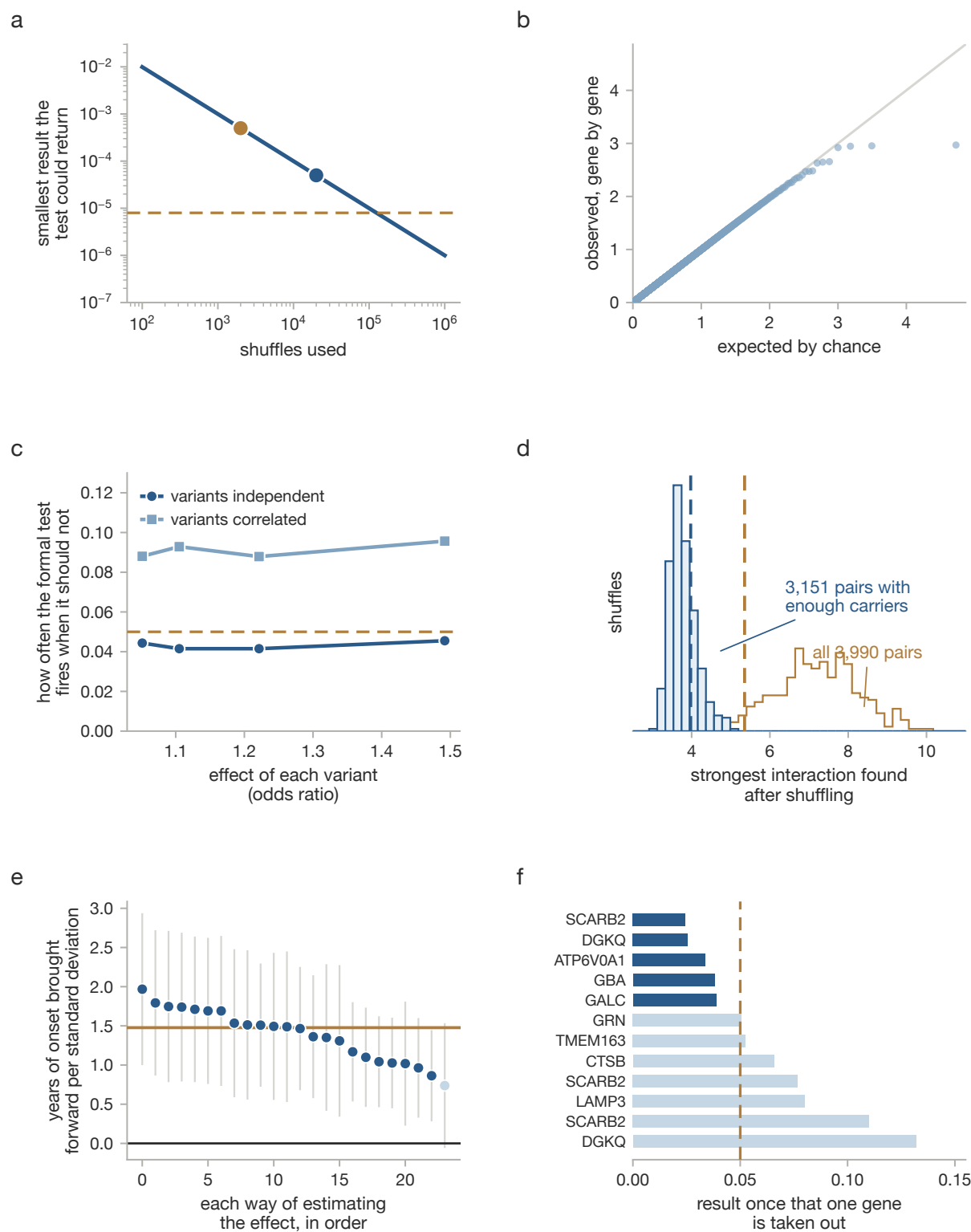
Supplementary Fig. 14 | Robustness diagnostics: permutation resolution ( a ), gene-level calibration ( b ), type-I error under linkage disequilibrium ( c ), the interaction null ( d ), the specification curve ( e ) and leave-one-out for the lysosomal enrichment ( f ).
