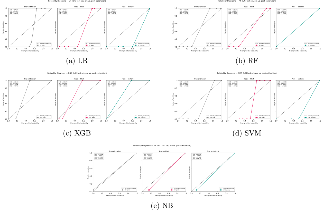
Figure 1: Reliability diagrams for all five classifiers before and after post-hoc calibration on the UCI test set. Each panel shows the uncalibrated model (grey), Platt scaling (pink), and isotonic regression (teal). The diagonal is perfect calibration. LR shows the largest pre-calibration deviation. Isotonic regression achieves the largest ECE reductions across the suite. Platt scaling raised SVM calibration error rather than reducing it.
