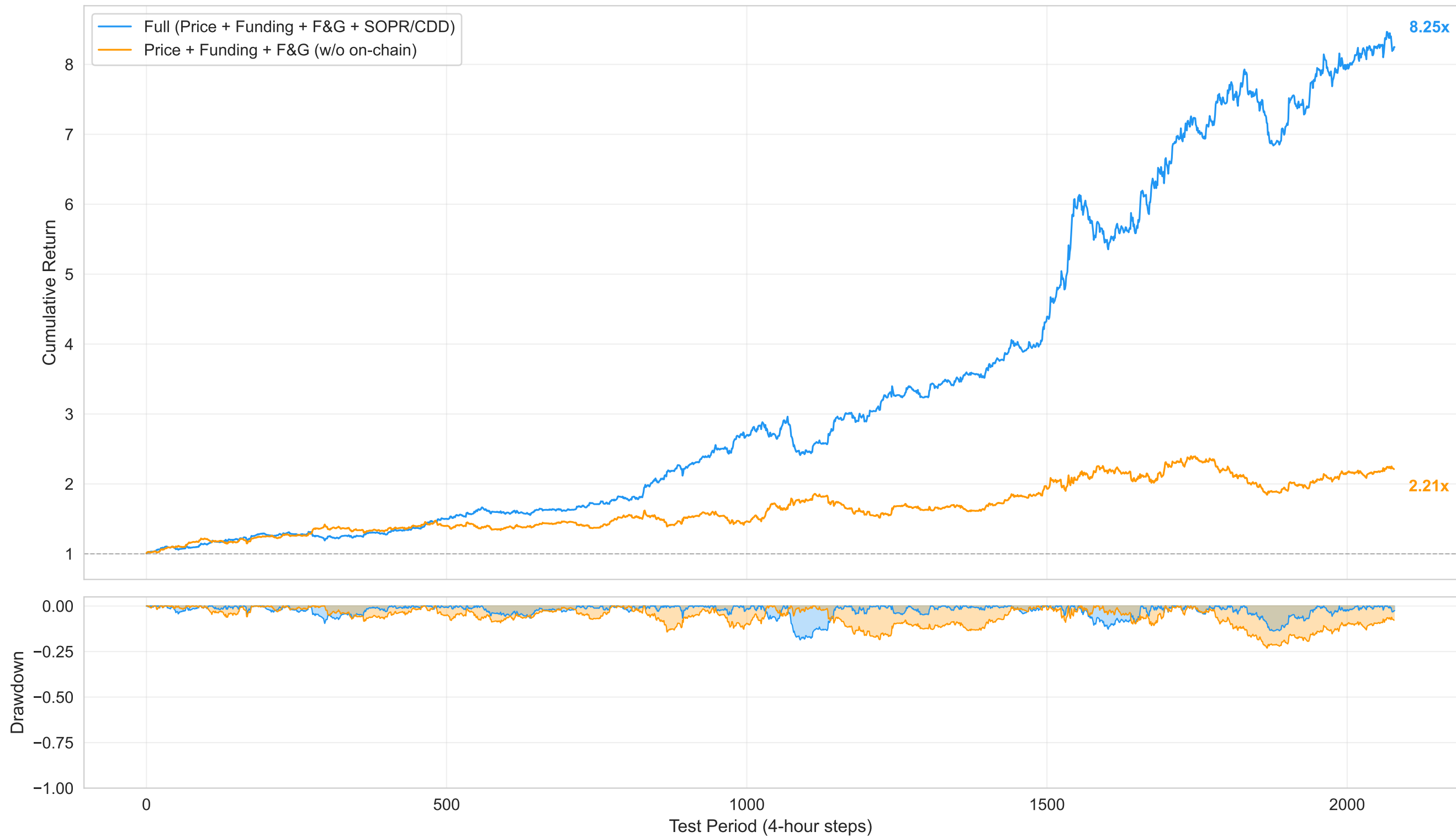
CNN-Transformer Backtest: Full vs Price+Funding+F&G (seed=1)
