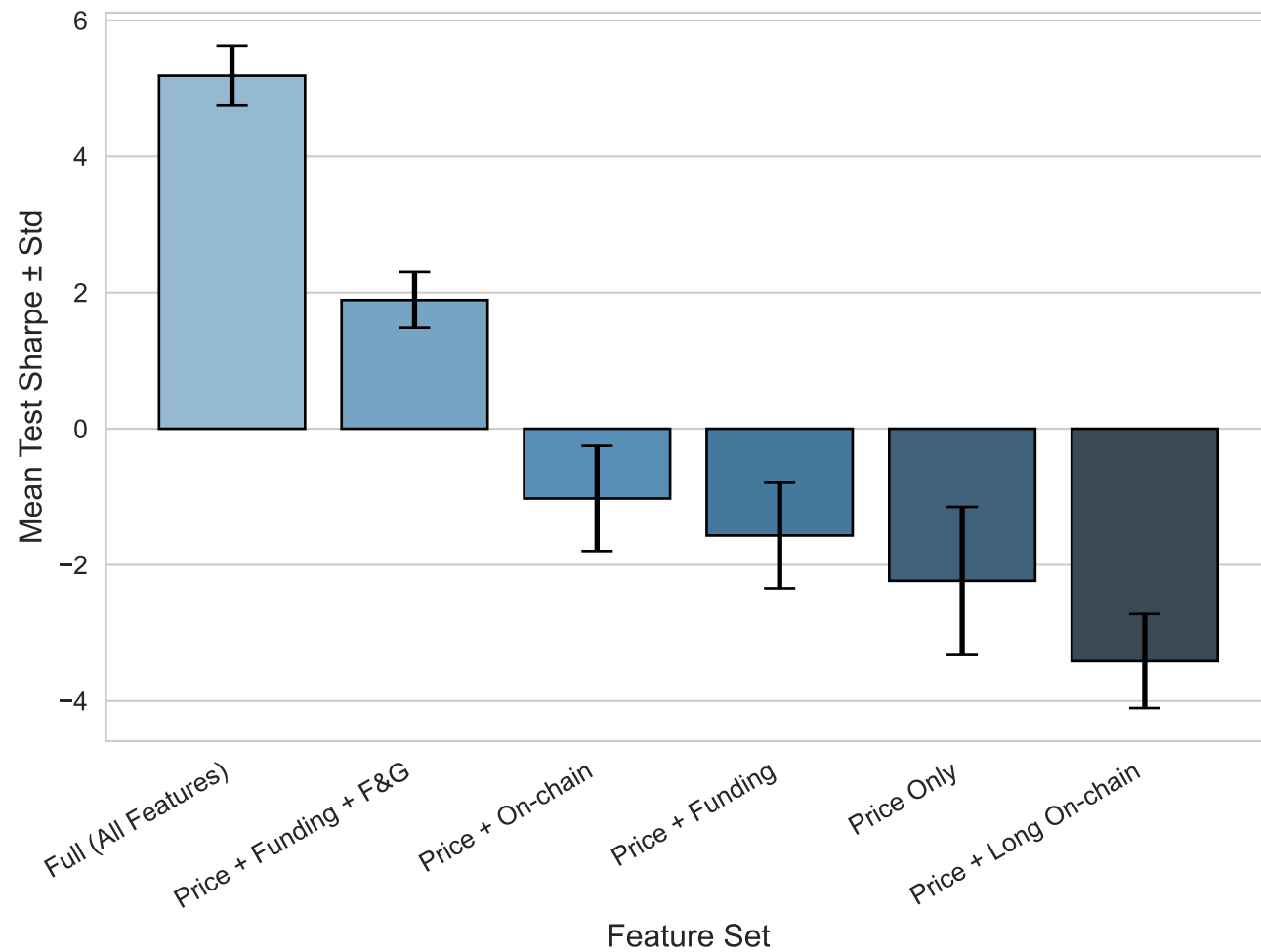
Test Sharpe (5 seeds)
