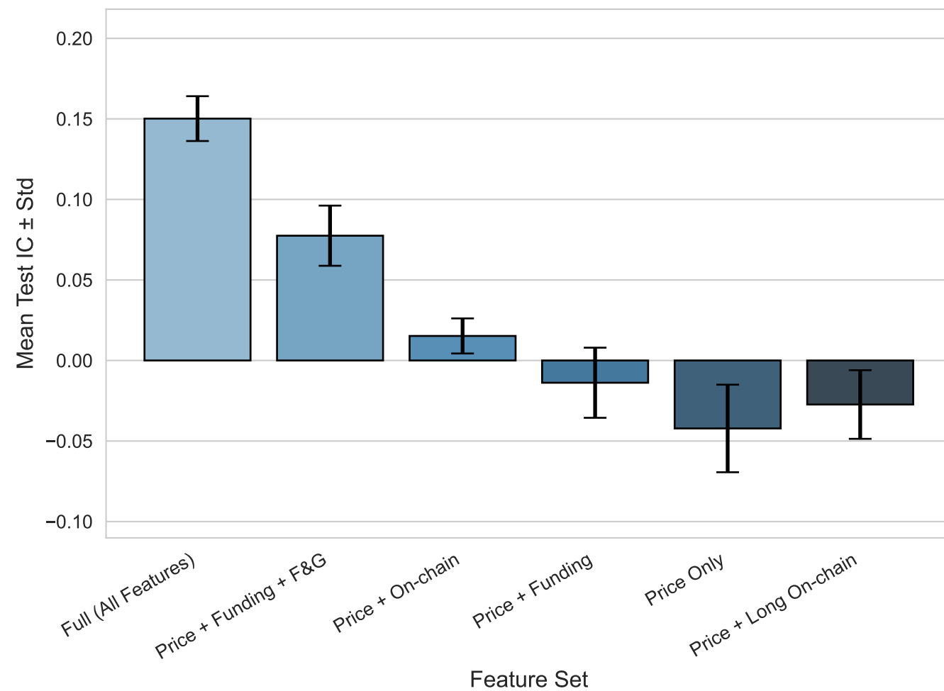
Test IC (5 seeds)
