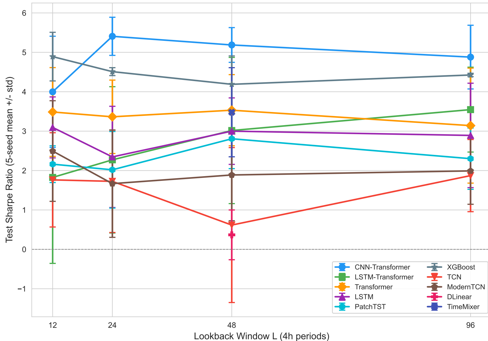
Test Sharpe vs Lookback Window
