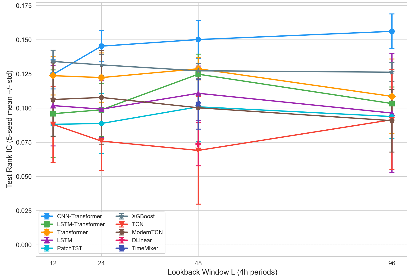
Test IC vs Lookback Window
