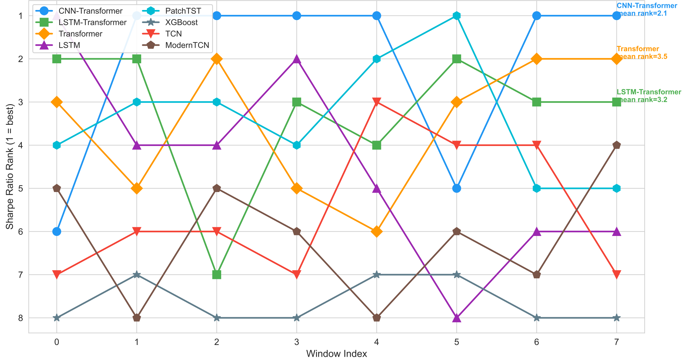
Model Rank Consistency Across Sliding Windows (Full Feature Set, Seed=1)
