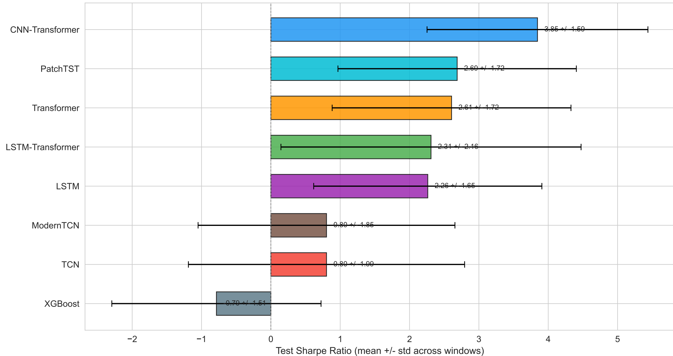
Model Stability Across Sliding Windows (Full Feature Set, Seed=1)
