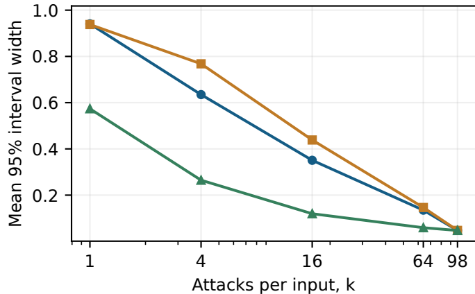
Logistic regression
