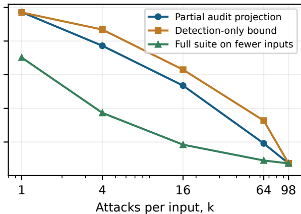
Random forest
