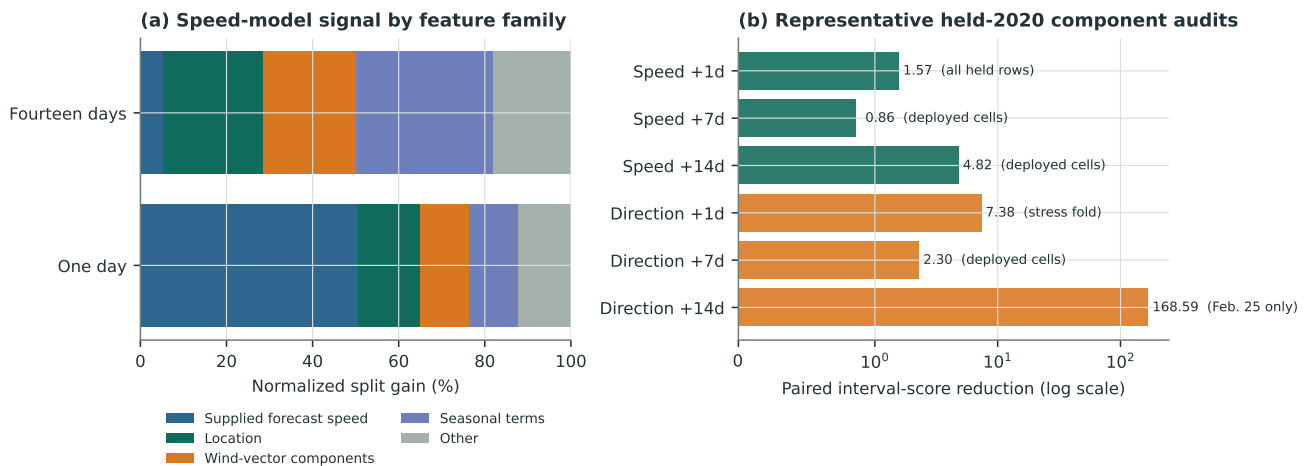
Figure 2: Model interpretation and validation audit. Panel (a) groups normalized split gain by feature family; it describes model use rather than causality. Panel (b) shows a representative held-2020 paired reduction for each target branch on that component’s activation mask. The logarithmic axis makes the sparse February-only fourteen-day direction audit visible without hiding the other five; magnitudes are not compared across masks.
