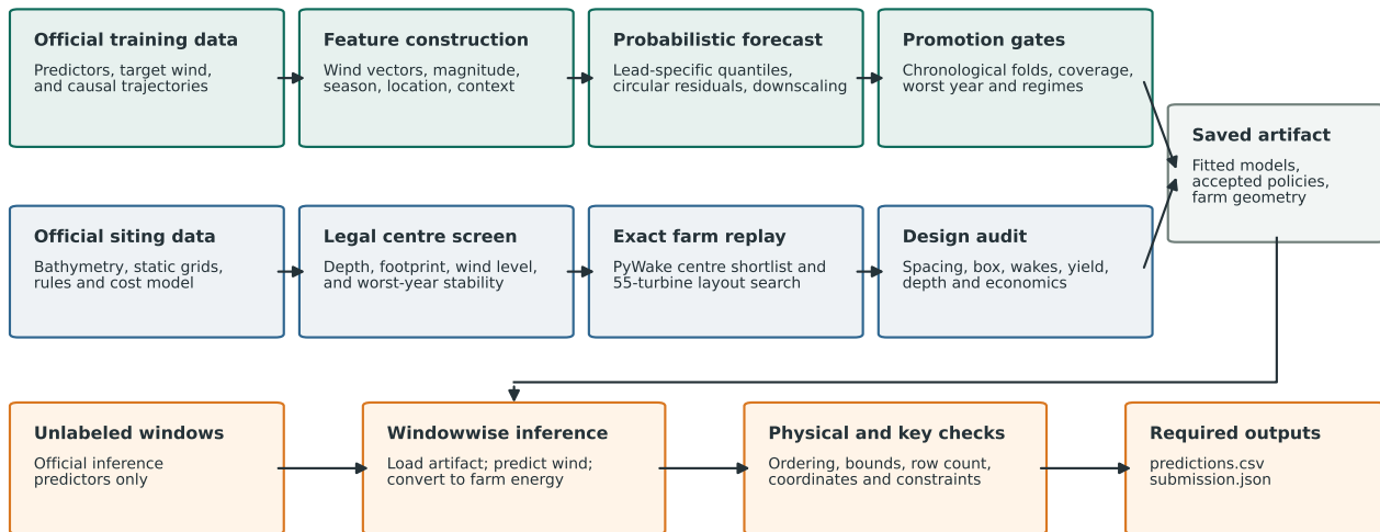
Figure 1: End-to-end generation pipeline. Labeled wind targets are confined to training and validation. Inference reads only the saved artifact and unlabeled official predictors.
