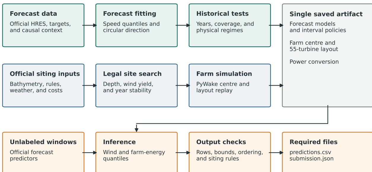
Figure 1: End-to-end generation pipeline. Labelled wind targets are confined to training and validation. Inference reads only the saved artifact and unlabelled official predictors.
