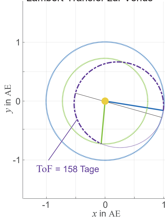
Lambert-Transfer zur Venus
