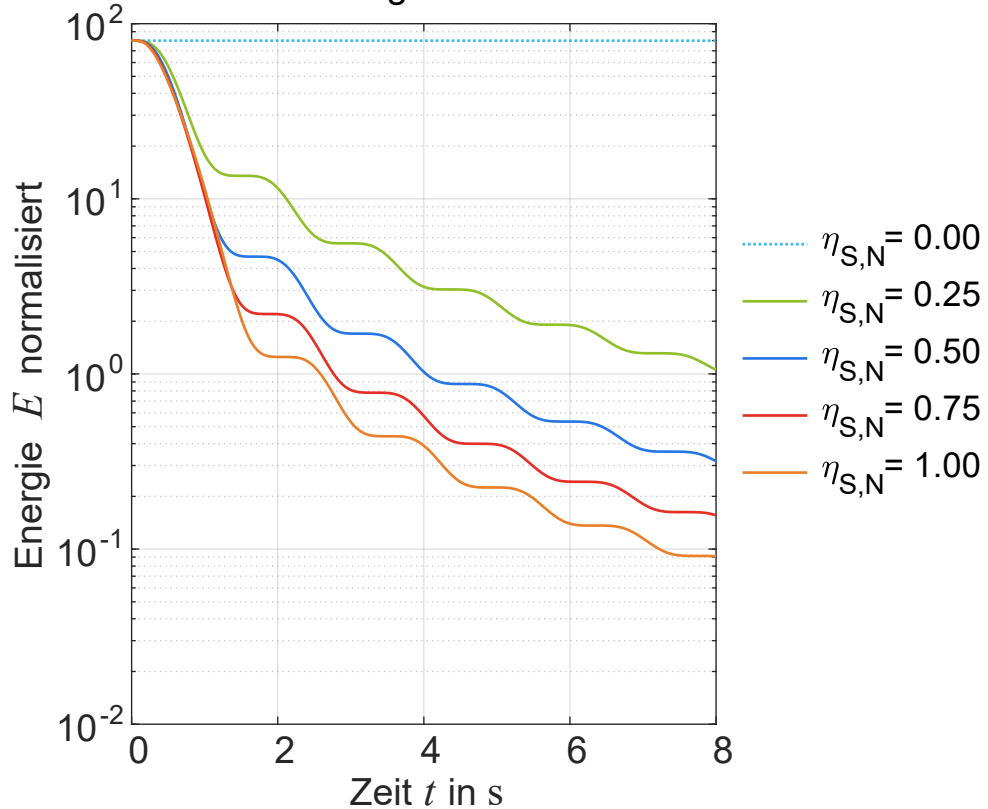
Newton-Reibung
