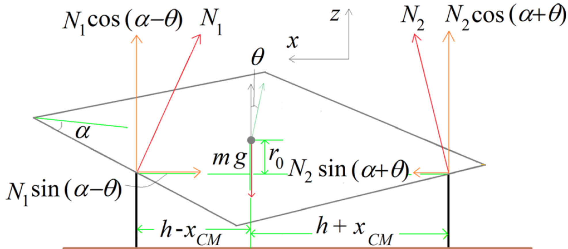
Fig. 4. Free body diagram of the cone, in the xz -plane (back view). The forces as well as their respective components can be seen. The forces are not to scale and labels indicate their magnitudes (the lines represent the directions). For the configuration shown here the angle \theta is negative.
