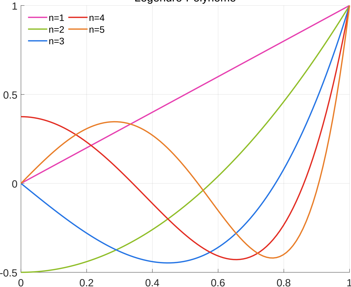
Legendre-Polynome
