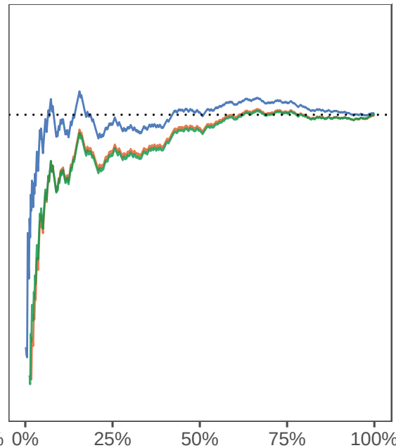
causal_forest
