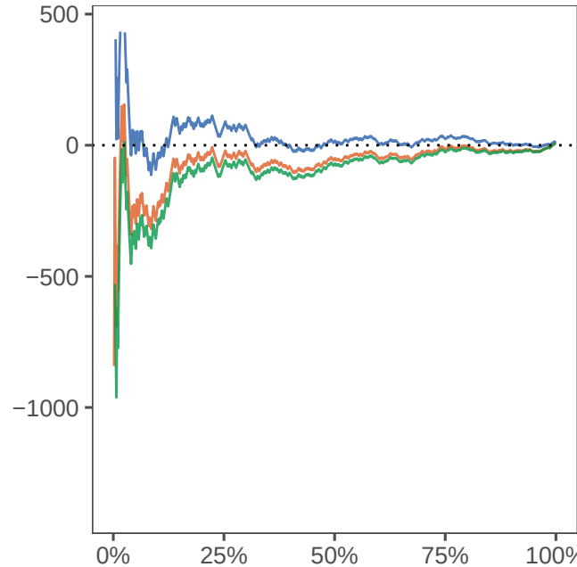
bartc
