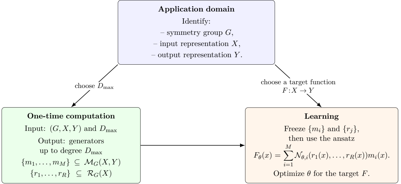
Figure 1: Proposed workflow for learning G -equivariant functions F : X \rightarrow Y . Starting from an application domain, one identifies the symmetry group G , the input representation X , and the output representation Y . For the resulting triple (G, X, Y) , one chooses a degree bound D_{\max} and performs a one-time computation of covariant generators \{m_1, \dots, m_M\} \subseteq \mathcal{M}_G(X, Y) and invariant generators \{r_1, \dots, r_R\} \subseteq \mathcal{R}_G(X) up to degree D_{\max} . For any G -equivariant target function F : X \rightarrow Y , one trains the neural network \mathcal{N}_\theta : \mathbb{R}^R \rightarrow \mathbb{R}^M in Eq. (2). In particular, for fixed (G, X, Y) , the same one-time computation can be reused to learn multiple G -equivariant functions from X to Y by training different neural networks.
