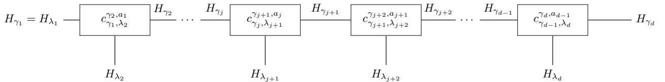
Figure 2: Tensor-network diagram for the tensor train in Eq. (9). Horizontal wires carry the intermediate irreps in the admissible path \gamma_1 \rightarrow \dots \rightarrow \gamma_d . Reading the contraction from right to left gives the map C_{\lambda, \gamma, \mathbf{a}} .
