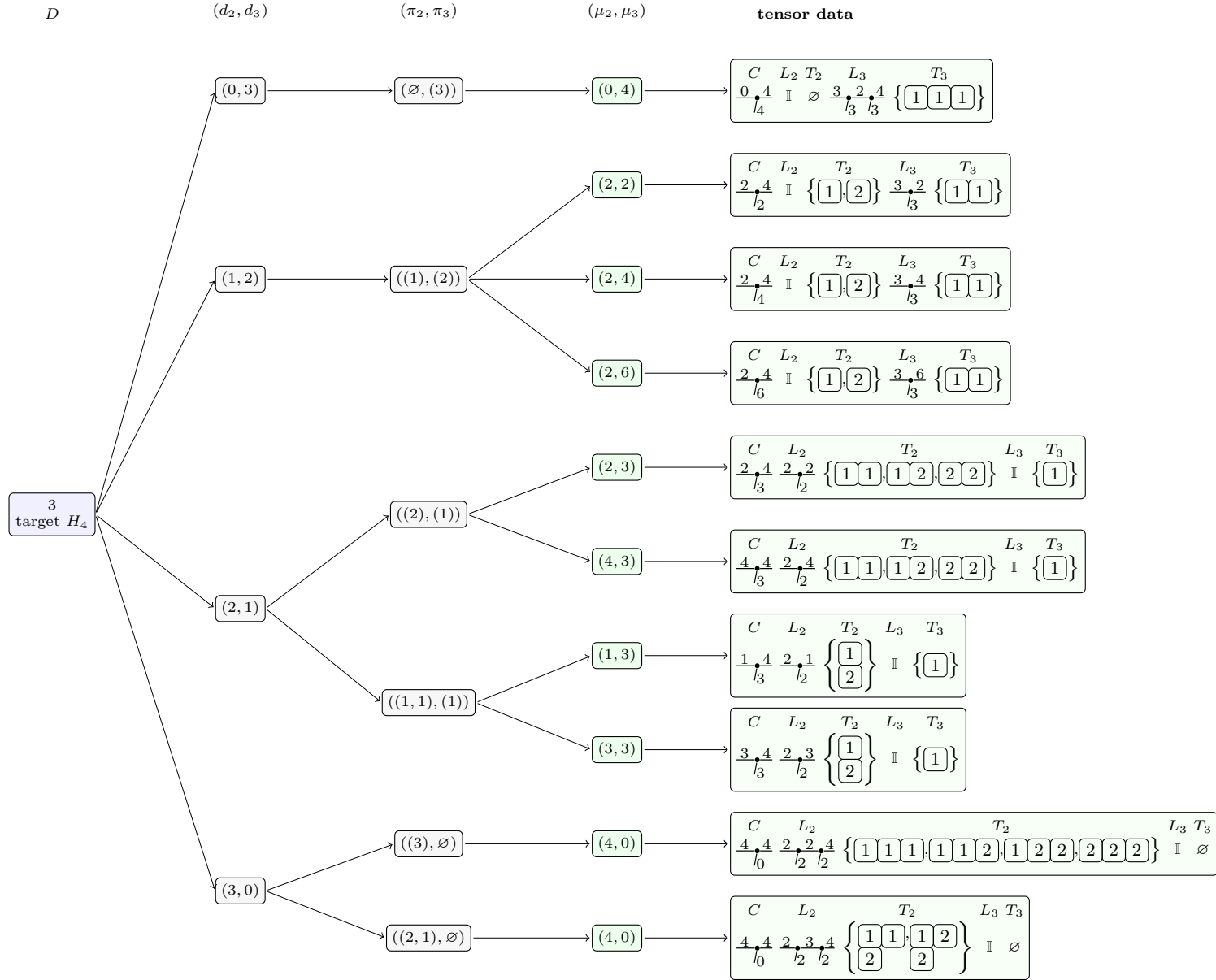
Figure 2: Condensed degree-3 isotypic data for X = 2H_2 \oplus H_3 and output H_4 .
