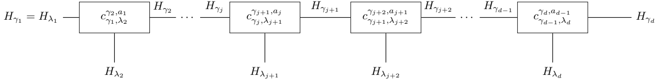
Figure 1: Tensor-network diagram for the tensor train in Eq. (7). Horizontal wires carry the intermediate irreps in the admissible path \gamma_1 \rightarrow \dots \rightarrow \gamma_d . Reading the contraction from right to left gives the map C_{\lambda, \gamma, \mathbf{a}} .
