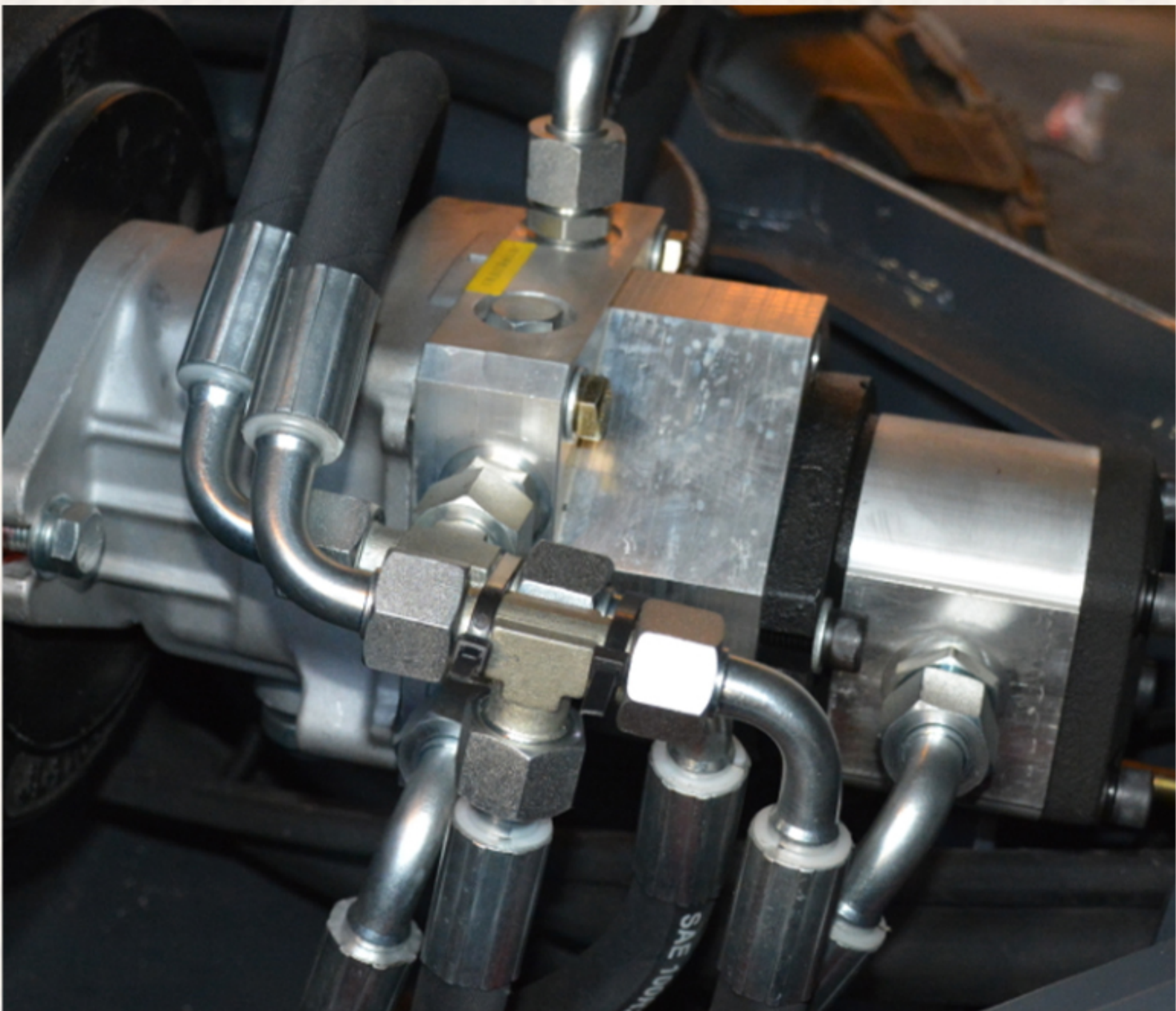
HYDROSTATIC SYSTEM
