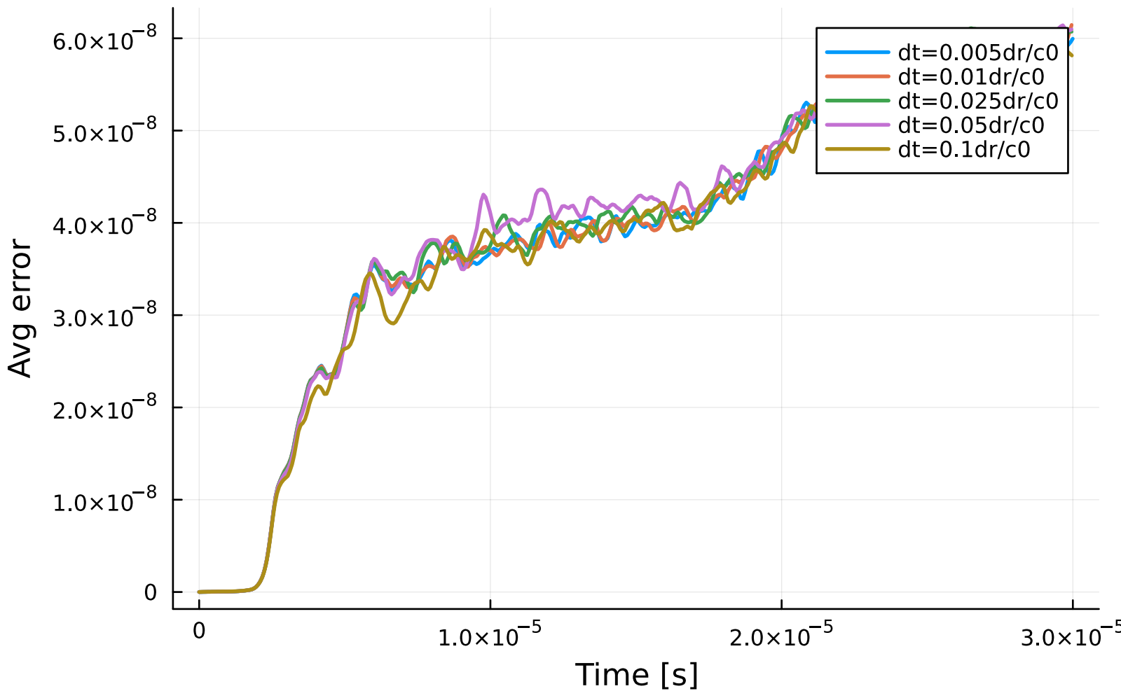
Avg error over time -- MLSEvolved, dr=0.00025
