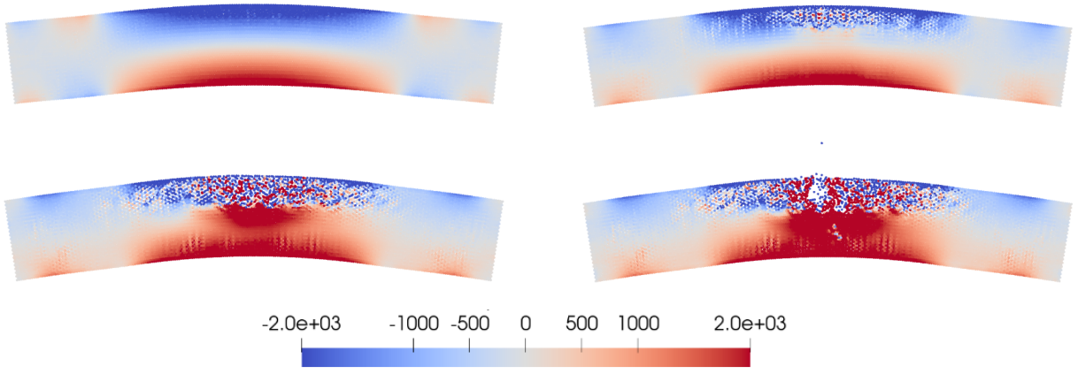
Figure 2: Pressure field of the projection of A - SingleSum. The simulation will develop instabilities early and fail as expected.
