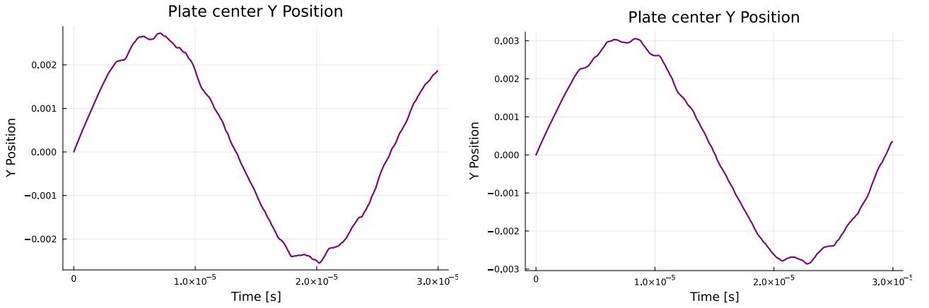
Figure 3: The y coordinate of the center point of the beryllium plate benchmark. (SingleSumEvolved left, MLSEvolved right)
