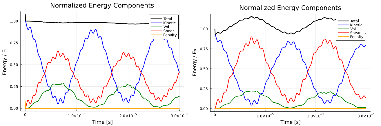
Figure 4: Normalized components of energy plotted against time. (SingleSumEvolved left, MLSEvolved right)
