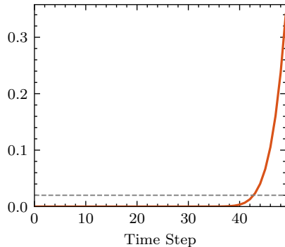
Additive Attention
