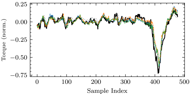
Difficult Prediction ( \text{MAE}_{M5}=0.038 )
