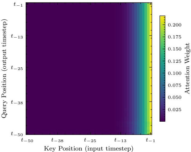
M7 Additive Attention
