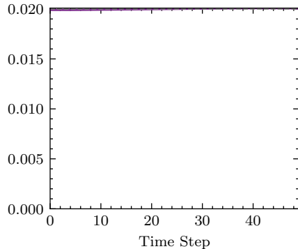
Scaled Dot-Product
