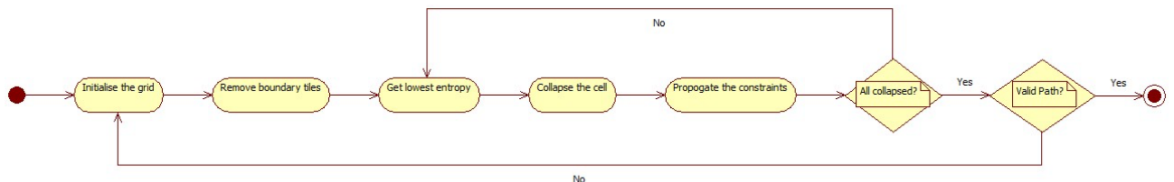
Figure 4-2 WFC Activity diagram
