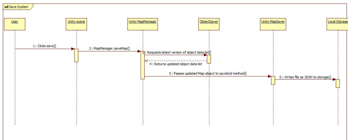
Sequence diagram of Save system
