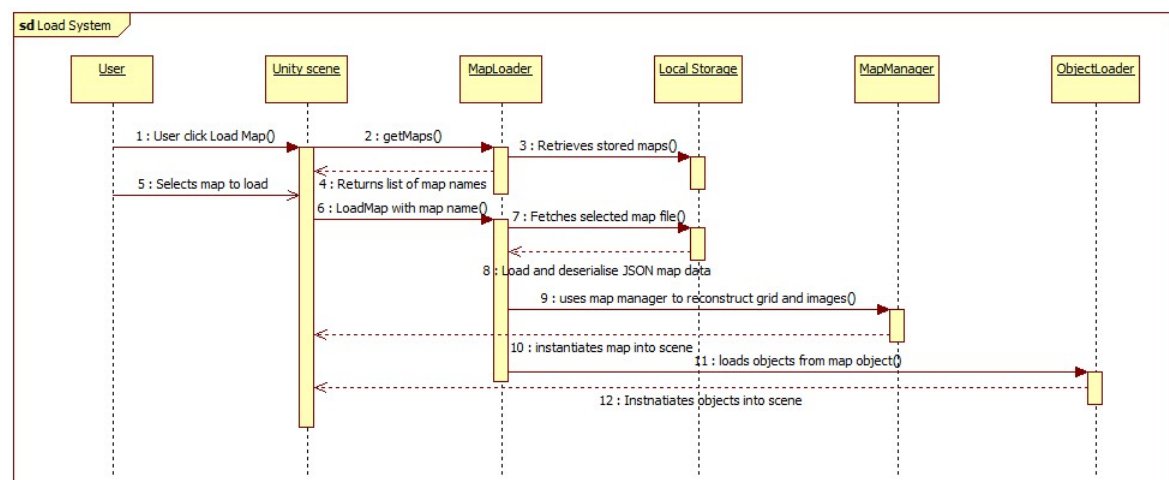
Sequence diagram of Load system
