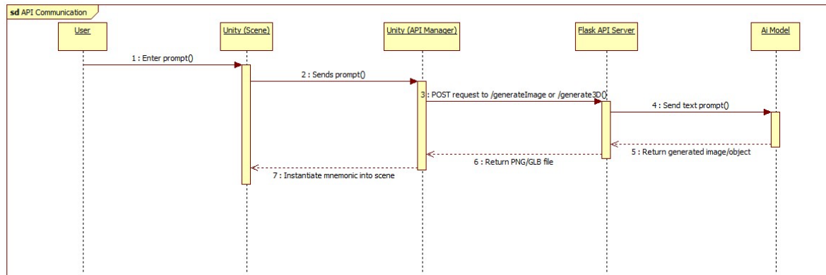
Sequence diagram of API communication
