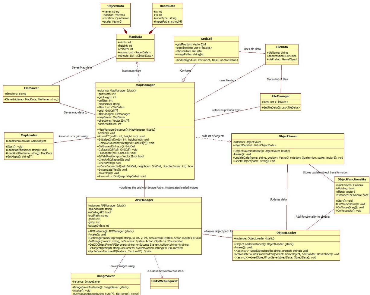
UML Class diagram
