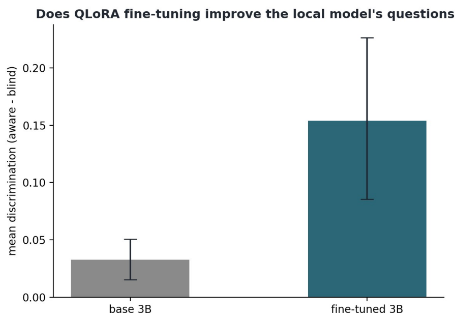
Figure 7.4: The QLoRA fine-tune of Qwen2.5 3B against its own base model on the same 18 claims, mean discrimination with 95 percent bootstrap intervals. The raw score rises from 0.033 to 0.154, but the quality audit in Section 8.9 shows this rise to be an artifact of degenerate output rather than better questions.
