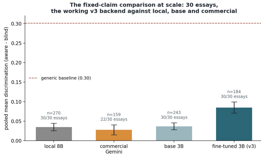
Figure 8.7: The fixed-claim comparison at thirty essays with the working v3 backend. All 856 questions are well-formed. v3 clears the base 3B ( p < 0.0001 ) and, on the 22 shared essays, the commercial model ( p = 0.0002 ); the commercial-versus-8B null replicates. Coverage is printed on each bar: the free-tier commercial arm covers 22 of 30 essays.
