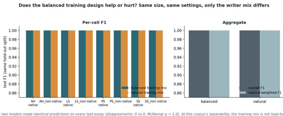
Figure 6.4: The training-distribution control. Two same-size detectors, one trained on the balanced writer mix and one on BAWE's natural skew, evaluated per cell and in aggregate on the same held-out split. The two are indistinguishable everywhere, so the balanced design does not explain why the corpus is separable.
