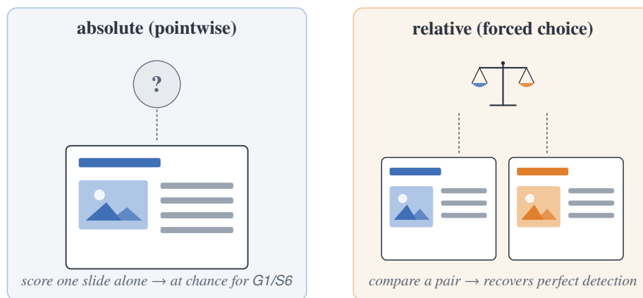
Figure 12: Two elicitation, same model and images. Pointwise (absolute) inspects one slide in isolation; the forced choice compares a pair. For G1 and S6, changing absolute to relative is what recovers detection (Sec. 4 of the main paper).
