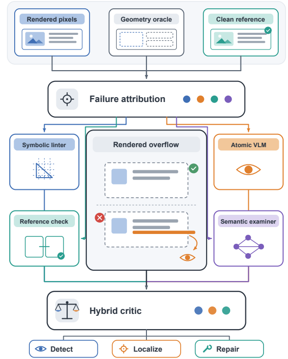
Figure 1: Diagnose before inspection. A geometry oracle attributes each failure and guides a manually specified division of labor among symbolic linting, atomic VLM elicitation, reference requests, and direct semantic inspection.
