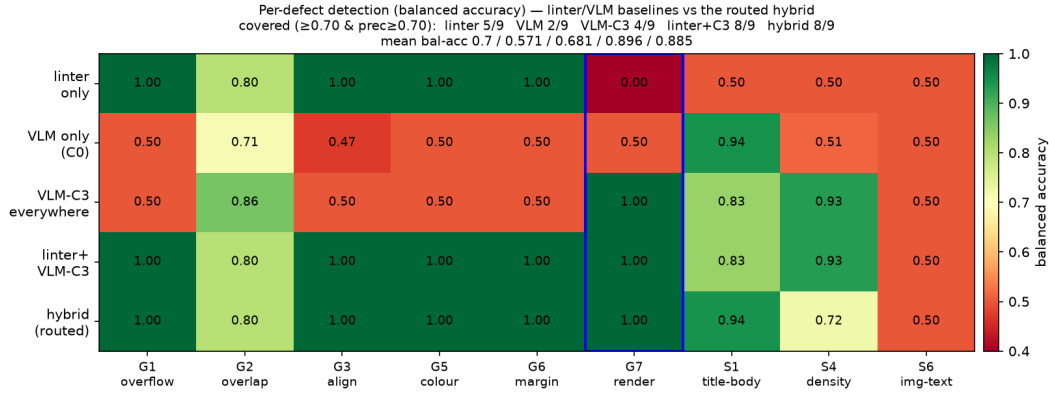
Figure 9: Coverage by engine. Per-defect balanced accuracy for the linter, VLM-C0, VLM-C3, linter+VLM-C3, and the routed hybrid. Minimal linter+C3 matches routed coverage; G7 (boxed) is the linter-blind cell rescued by C3.
