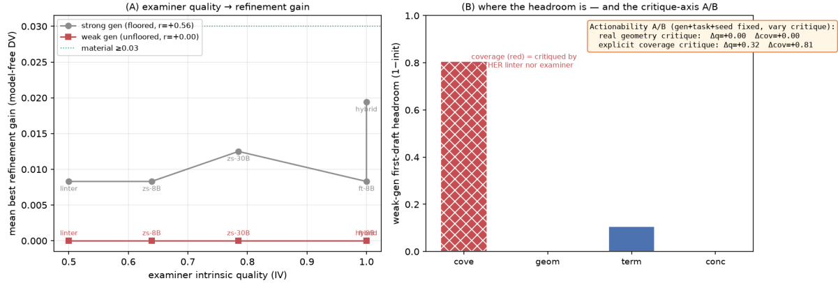
Figure 9: Unfloored downstream (E6): more headroom, no gain—a critique-axis mismatch. (A) examiner intrinsic quality vs. best refinement gain on a model-free quality. The strong (floored) generator gives the hypothesised slope ( r=+0.56 ) at tiny magnitude; the weak generator—despite 1.43\times the first-draft headroom—is flat ( r=0.00 ), no condition reaching the material threshold. (B) the weak generator’s headroom by dimension is dominated by coverage (red), which neither the linter nor the examiner critiques; the inset actionability A/B (same generator/task/seed, only the critique varies) shows the real geometry critique recovers nothing ( \Delta q=+0.00 ) while an explicit coverage critique recovers \Delta q=+0.32 ( \Delta cov=+0.81 )—so the null is an axis mismatch, not an inability to revise.
