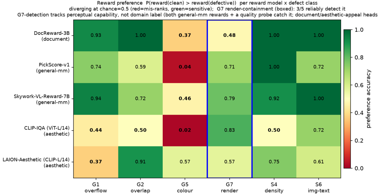
Figure 6: G7-detection tracks perceptual capability, not the training-domain label. Preference accuracy per reward model \times defect class (green = sensitive, red = mis-ranks; chance = 0.5), five scorers, two per audited category. Every scorer is sensitive to several in-taxonomy classes, but for the boxed G7 render class detection splits by capability : both general-multimodal rewards (Skywork-VL 0.79, PickScore 0.71, distinct backbones) and the zero-shot perceptual-quality probe (CLIP-IQA 0.83) catch it, while the document reward (DocReward 0.48) and the artistic-aesthetic head (LAION 0.57) sit at chance—so the blind spot belongs to specialised critics, and is caught by any perceptually-capable scorer (prompted VLM, VL reward, or CLIP quality read).
