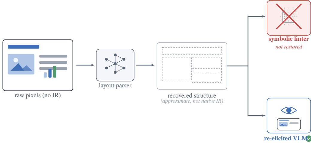
Figure 12: Open world: recovered structure does not restore the linter. For bare third-party pixels with no IR, a layout parser recovers approximate structure, but it is not the native IR the symbolic linter needs; only the re-elicited VLM remains a deployable critic (quantified in Fig. 13).
