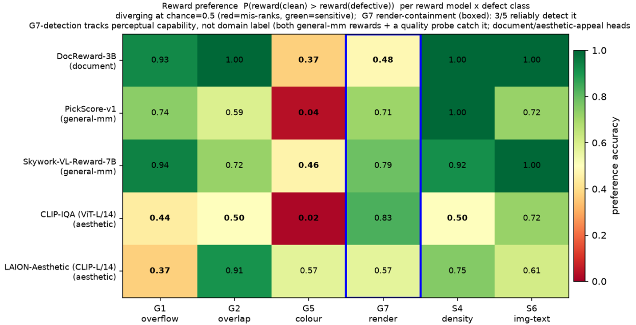
Figure 7: G7-detection tracks perceptual capability, not the training-domain label. Preference accuracy per reward model \times defect class (green = sensitive, red = mis-ranks; chance = 0.5), five scorers, two per audited category. Every scorer is sensitive to several in-taxonomy classes, but for the boxed G7 render class detection splits by capability : both general-multimodal rewards (Skywork-VL 0.79, PickScore 0.71, distinct backbones) and the zero-shot perceptual-quality probe (CLIP-IQA 0.83) catch it, while the document reward (DocReward 0.48) and the artistic-aesthetic head (LAION 0.57) sit at chance—so the blind spot belongs to specialised critics, and is caught by any perceptually-capable scorer (prompted VLM, VL reward, or CLIP quality read).
