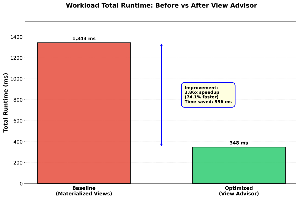
Figure 4.5.: Total Workload Runtime: Baseline vs. Advisor Recommendations
