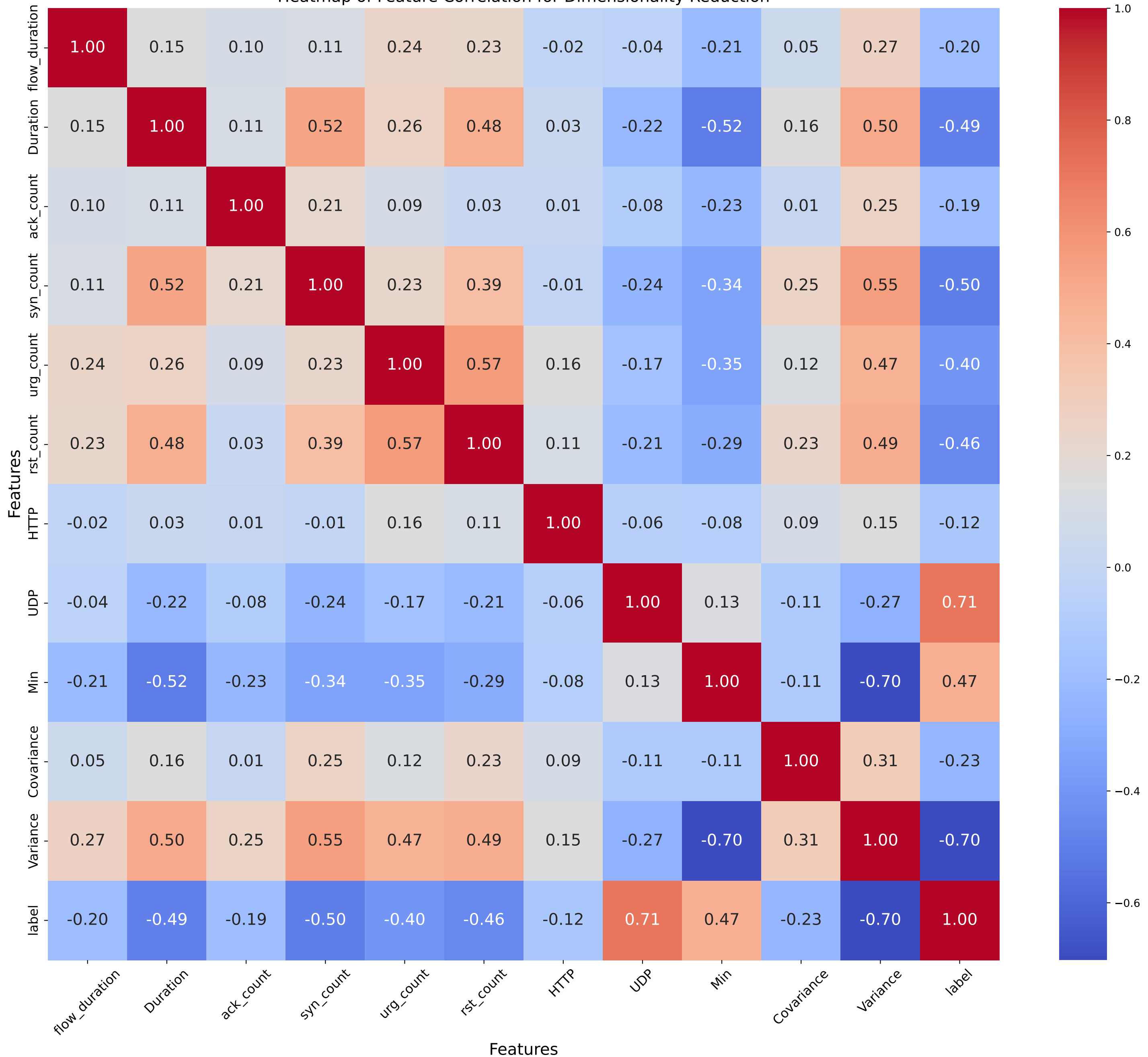
Heatmap of Feature Correlation for Dimensionality Reduction
