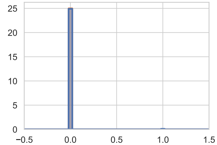
Feature: UDP
