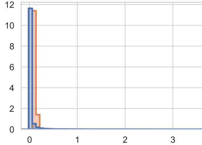
Feature: flow_duration
