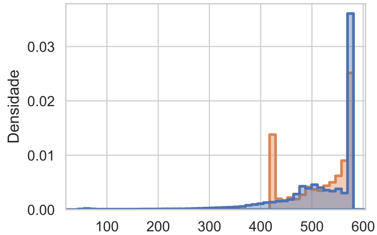
Feature: Min
