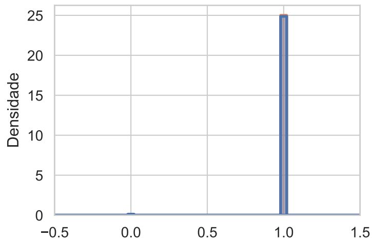
Feature: UDP
