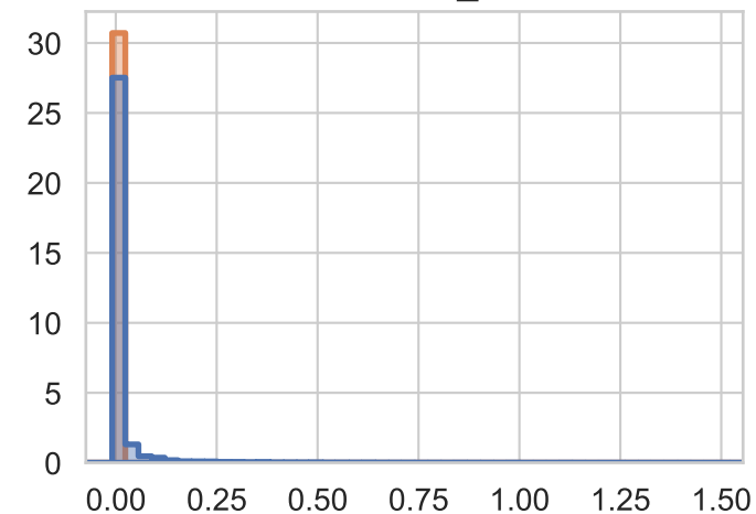
Feature: rst_count
