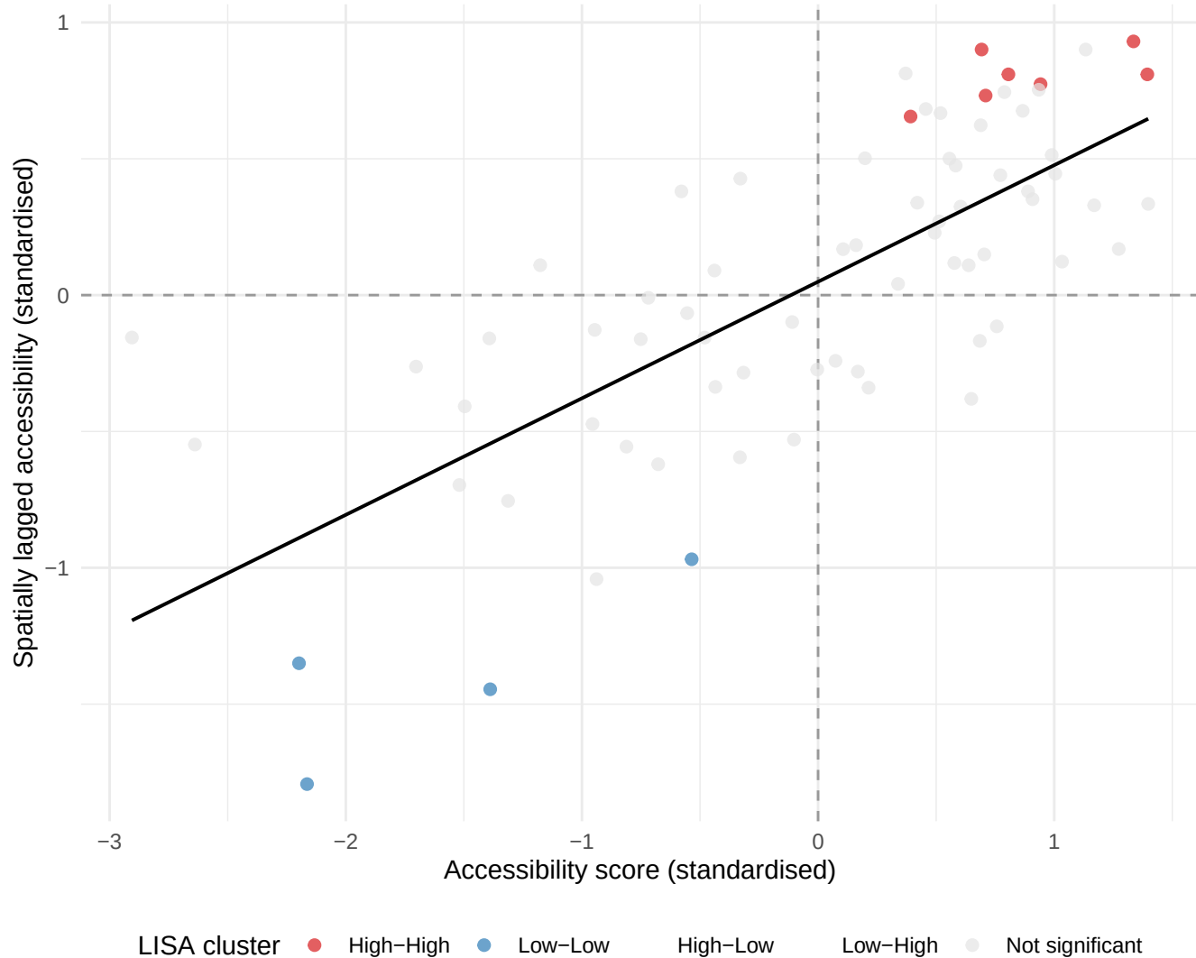
Moran Scatter Plot: Accessibility Score
