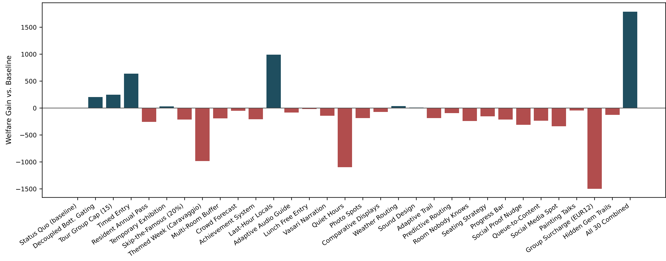
Intervention Comparison
