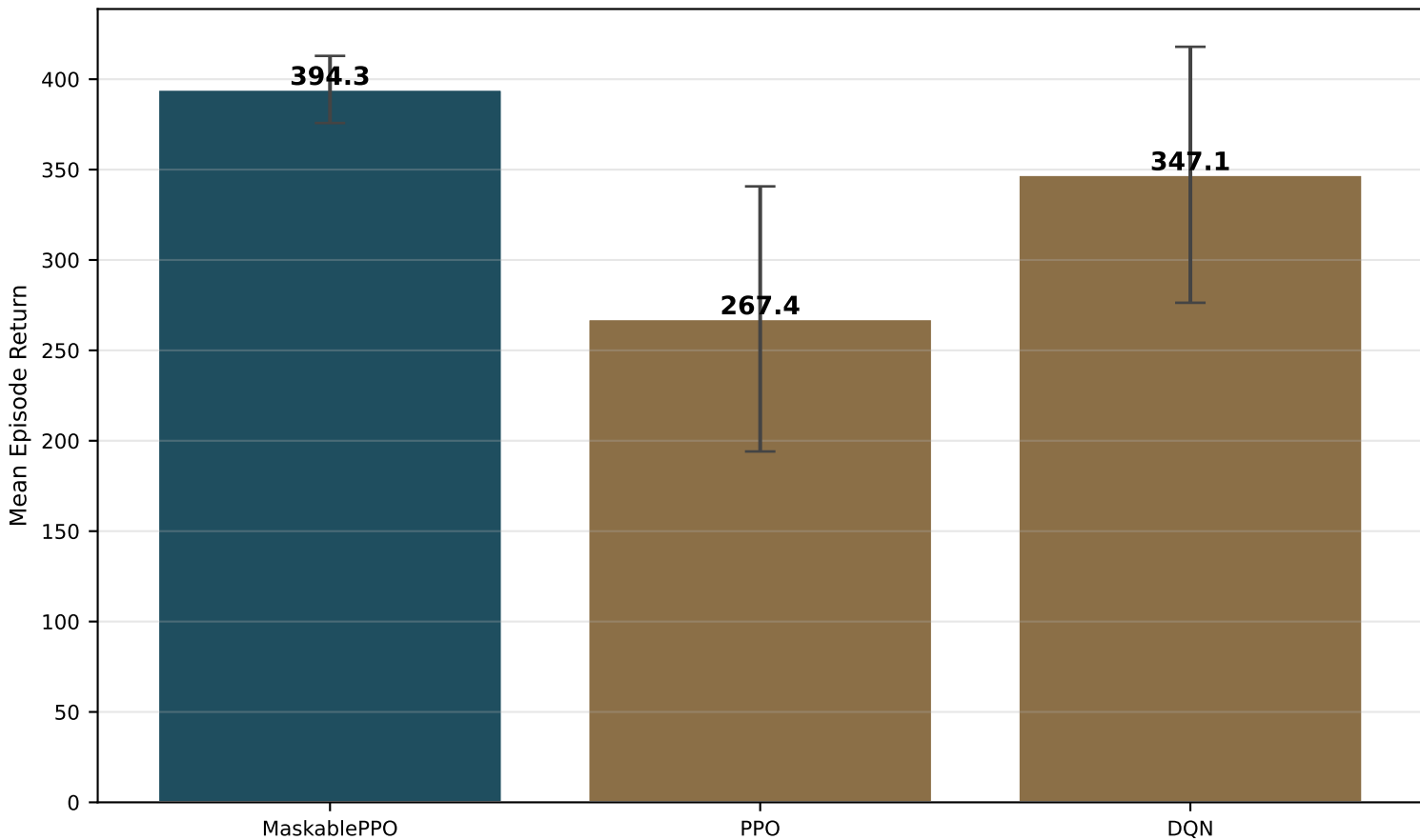
Deep RL Comparison on the Full 98-Room Museum
