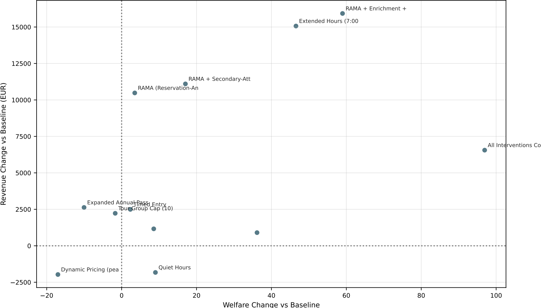
Welfare-Revenue Trade-off Across Interventions
