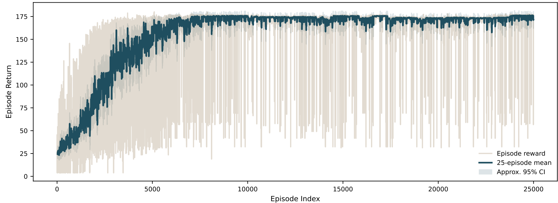
Tabular Q-Learning on Toy Graph
