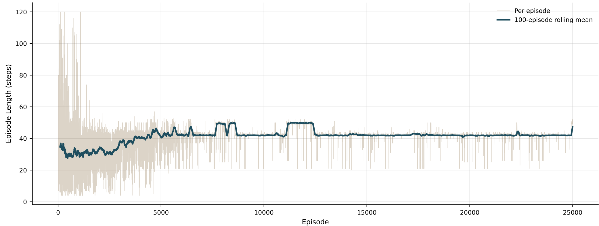
Episode Length Evolution During Q-Learning
