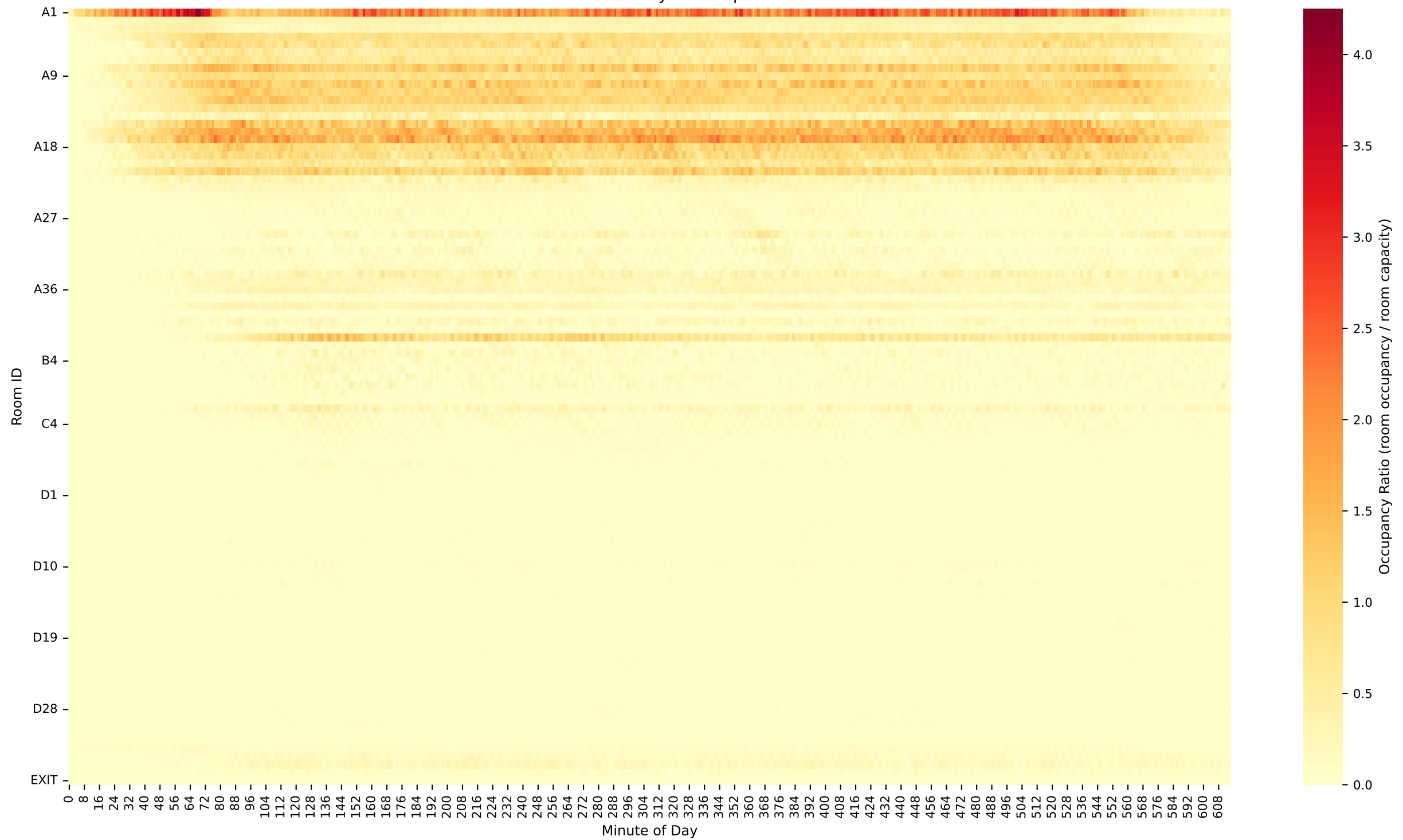
Crowd Density Heatmap
