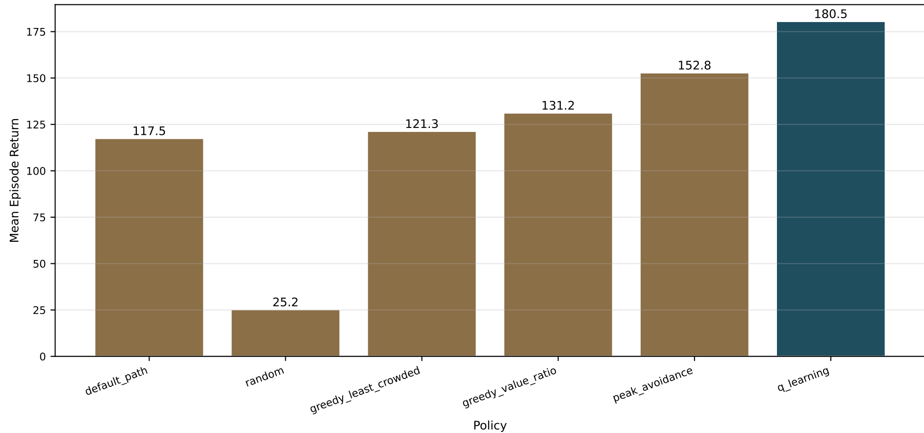
Q-Learning vs Handcrafted Baselines (12-Room Toy Graph)
