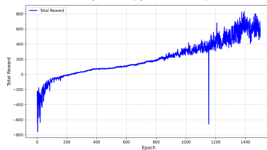
Episode Reward (BipedalWalkerHardcore-v3)
