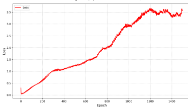
Training Loss (BipedalWalkerHardcore-v3)
