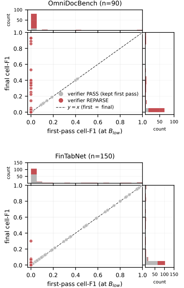
Fig. 3. Per-page first-pass vs. final cell-F1 for the adaptive system, colored by the verifier’s actual decision. Gray (PASS) pages lie on the diagonal by construction; the first pass is kept. Red (REPARSE) pages above the diagonal gained from the second pass; most OmniDocBench gains start from a first-pass score of zero, consistent with the NO_TABLE_FOUND-dominated trigger profile. No page fell below the diagonal in these runs. Stacked marginal histograms (top: first-pass, right: final; same color coding) expose the mass that overplots at the origin: 78/90 OmniDocBench and 93/150 FinTabNet first passes score zero, dropping to 58 and 87 at the final margin as escalation lifts 20 and 6 pages off the floor (cf. Table IV). Points are not jittered, so the diagonal relation is exact.
