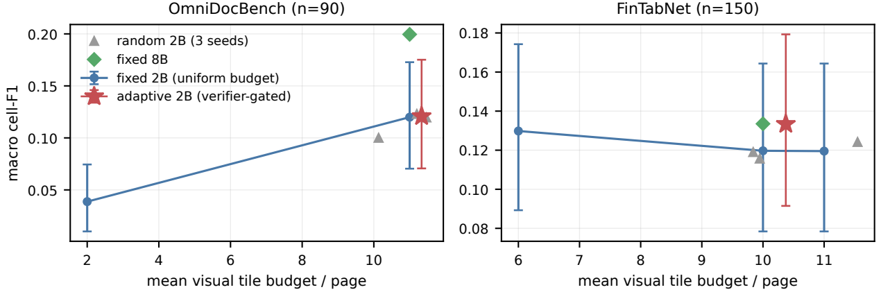
Fig. 2. Macro cell-F1 against mean tile budget. The two datasets respond to uniform budget in opposite ways. OmniDocBench (left) rises steeply from 2 to 11 tiles, and the adaptive policy lands on the fixed-budget line: selective escalation has nothing to add when uniform spending already pays. FinTabNet (right) is flat to slightly negative from 6 to 11 tiles; more uniform budget does not help. Yet the verifier-gated system sits above every same-cost 2B alternative and at the level of the tile-matched 8B reference. Error bars are marginal per-system 95% bootstrap CIs (percentile, 1000 resamples); the gray triangles plot all three random-control seeds individually, each the per-seed mean over pages, not a pooled mean. The significant adaptive-versus-random result is a paired per-page test (Table III) and is not represented by the overlap of these marginal intervals.
