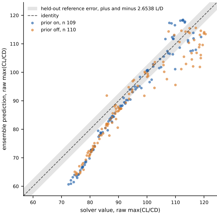
Figure 8. Surrogate against solver, admitted generated shapes
