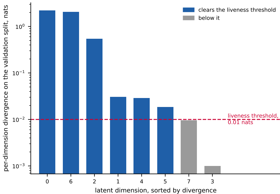
Figure A2. Latent dimension usage
